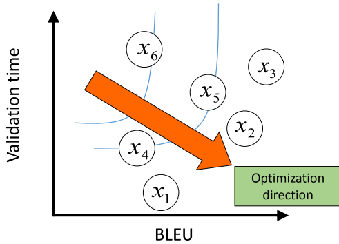
Figure 2: Pareto based optimization for two objectives.
