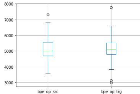
(b) Multi objective, BPE
