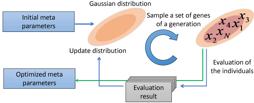
Figure 1: Automatic system tuning process using CMA-ES.
